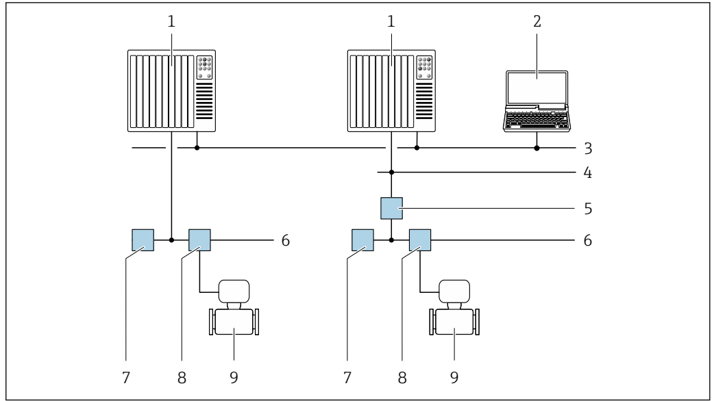
41 Options for remote operation via FOUNDATION Fieldbus network
