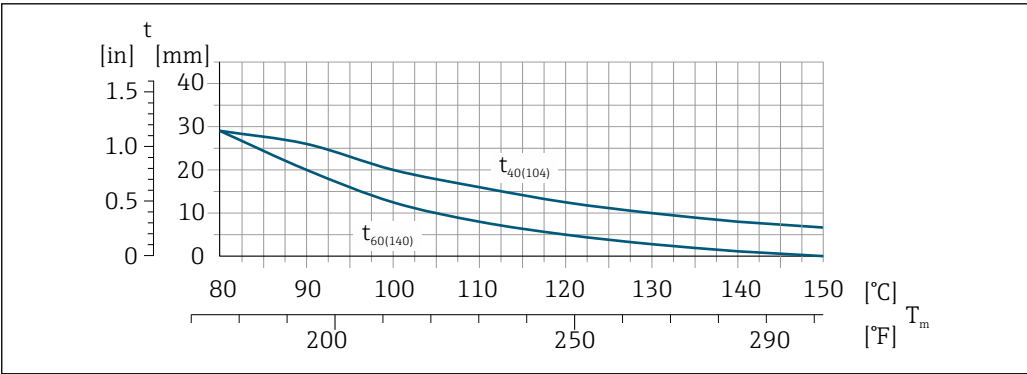
30 Maximum recommended insulation thickness depending on the temperature of the medium and the ambient temperature
