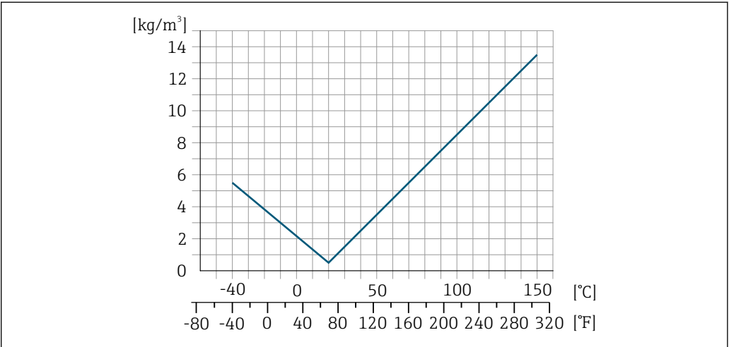
17 Field density calibration, for example at +20 ^\circ\text{C} (+68 ^\circ\text{F} )
