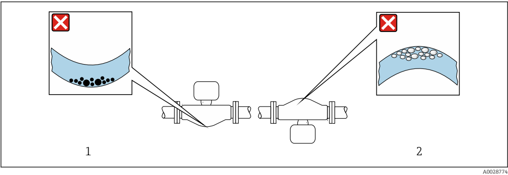
☒ 19 Orientation of sensor with curved measuring tube
